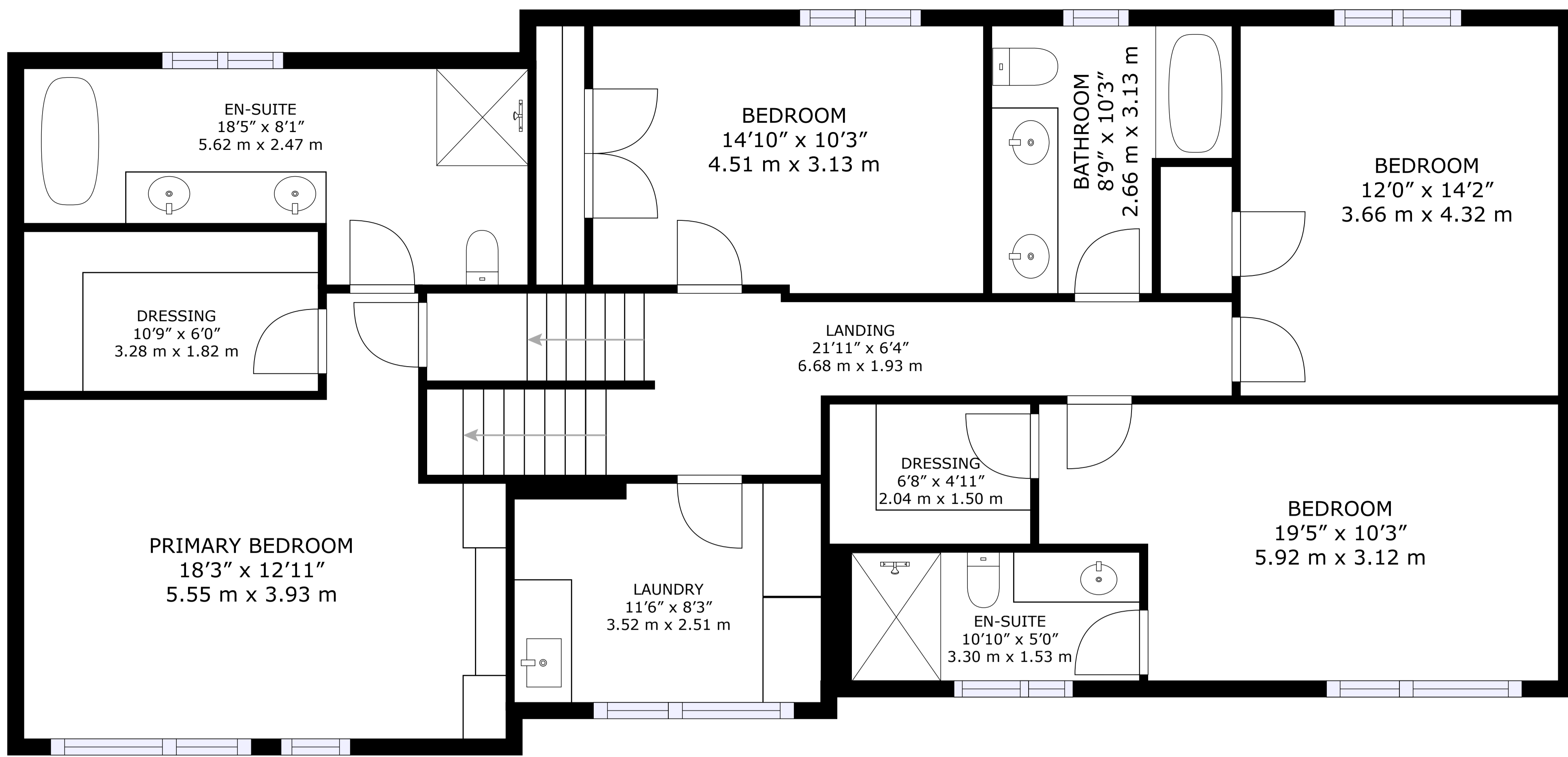
3RD FLOOR
