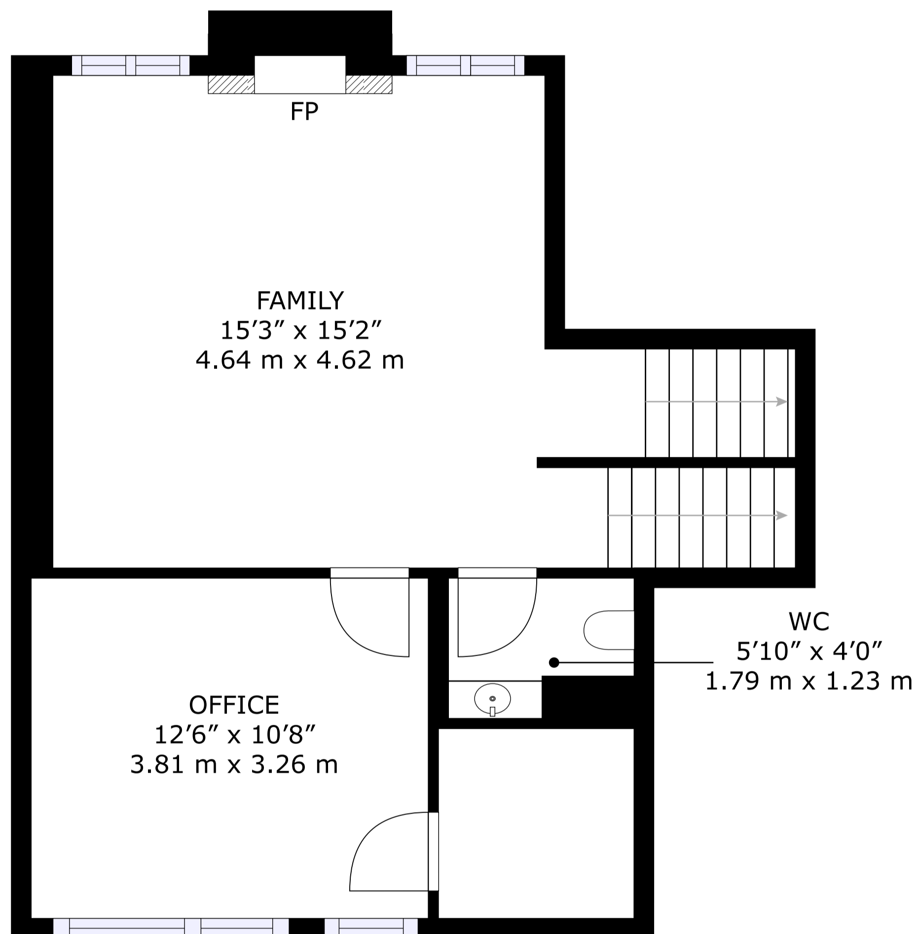
2ND FLOOR
